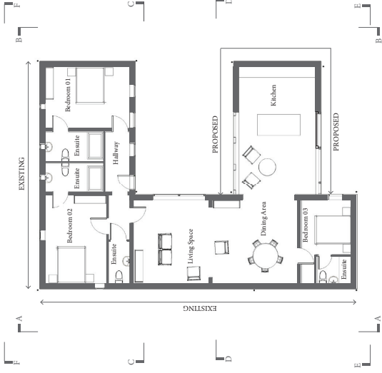
Ground Floor Plan 1:100@A1
